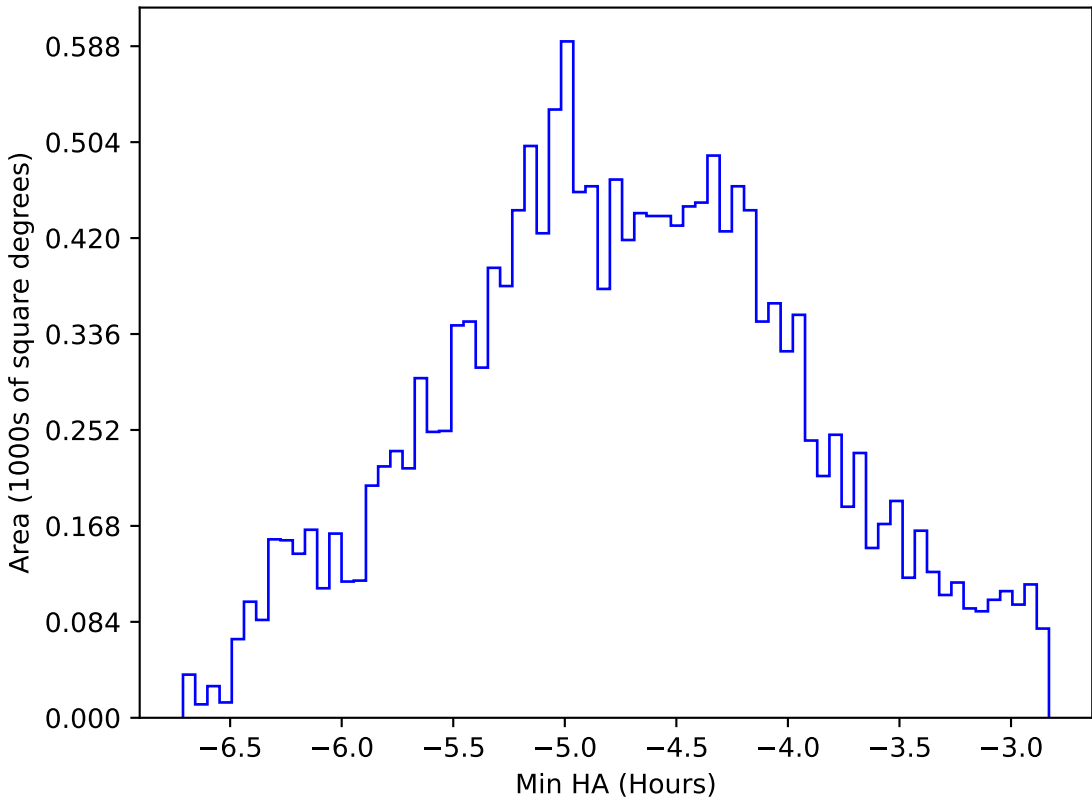
internal_u_expt30_nscale1.1v3.4_10yrs WFD all bands: Min HA
