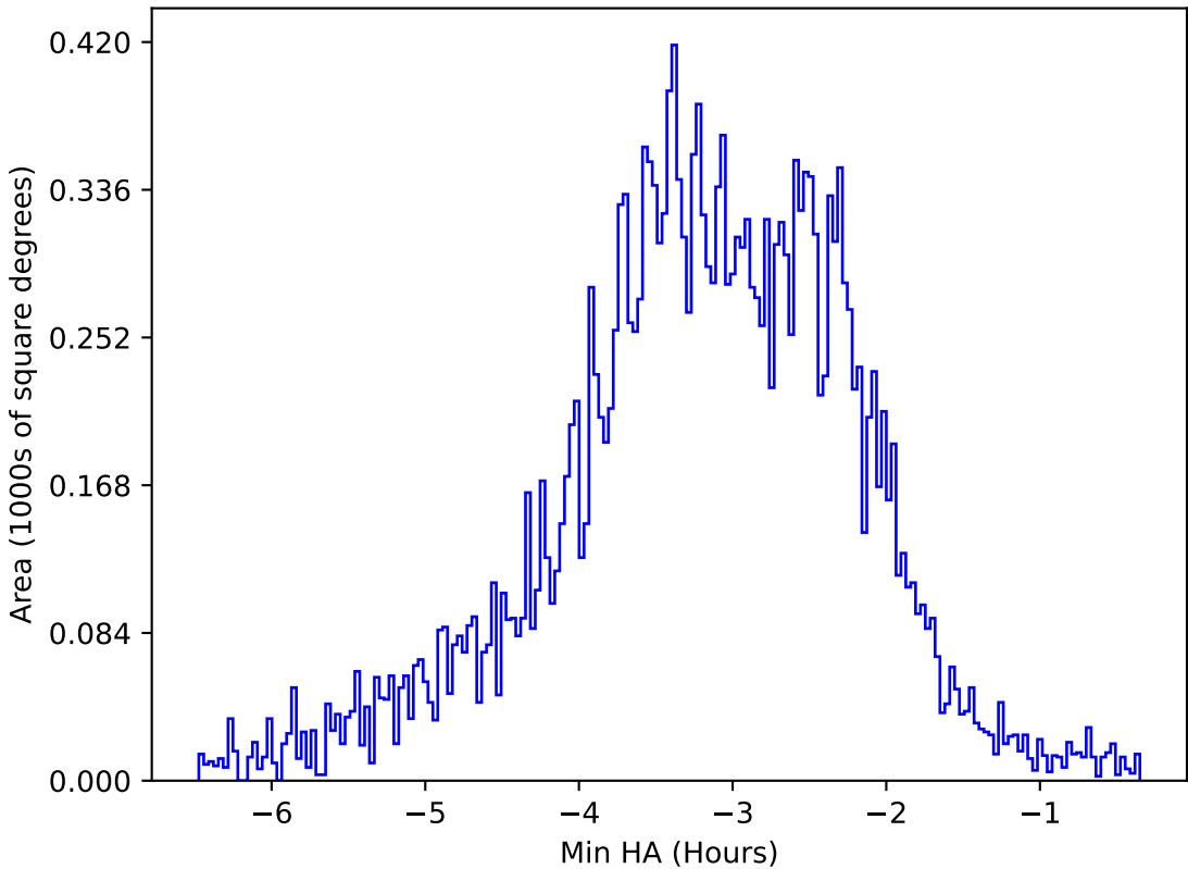
internal_u_expt30_nscale1.1v3.4_10yrs All sky u band: Min HA
