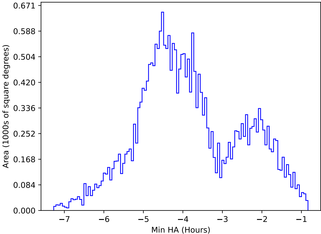
internal_u_expt30_nscale1.1v3.4_10yrs All sky g band: Min HA
