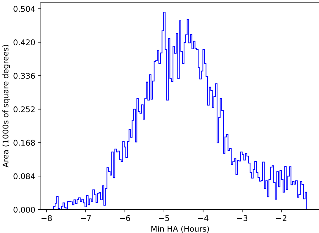
internal_u_expt30_nscale1.1v3.4_10yrs All sky all bands: Min HA
