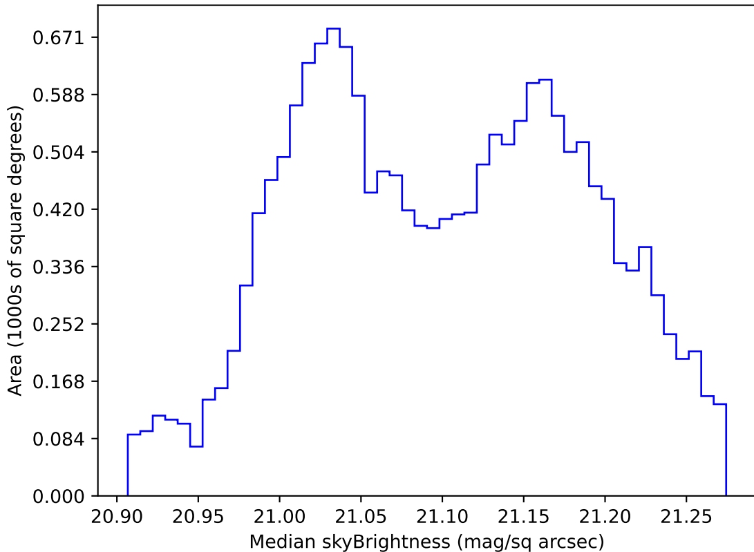
internal_u_expt30_nscale1.1v3.4_10yrs WFD r band: Median skyBrightness
