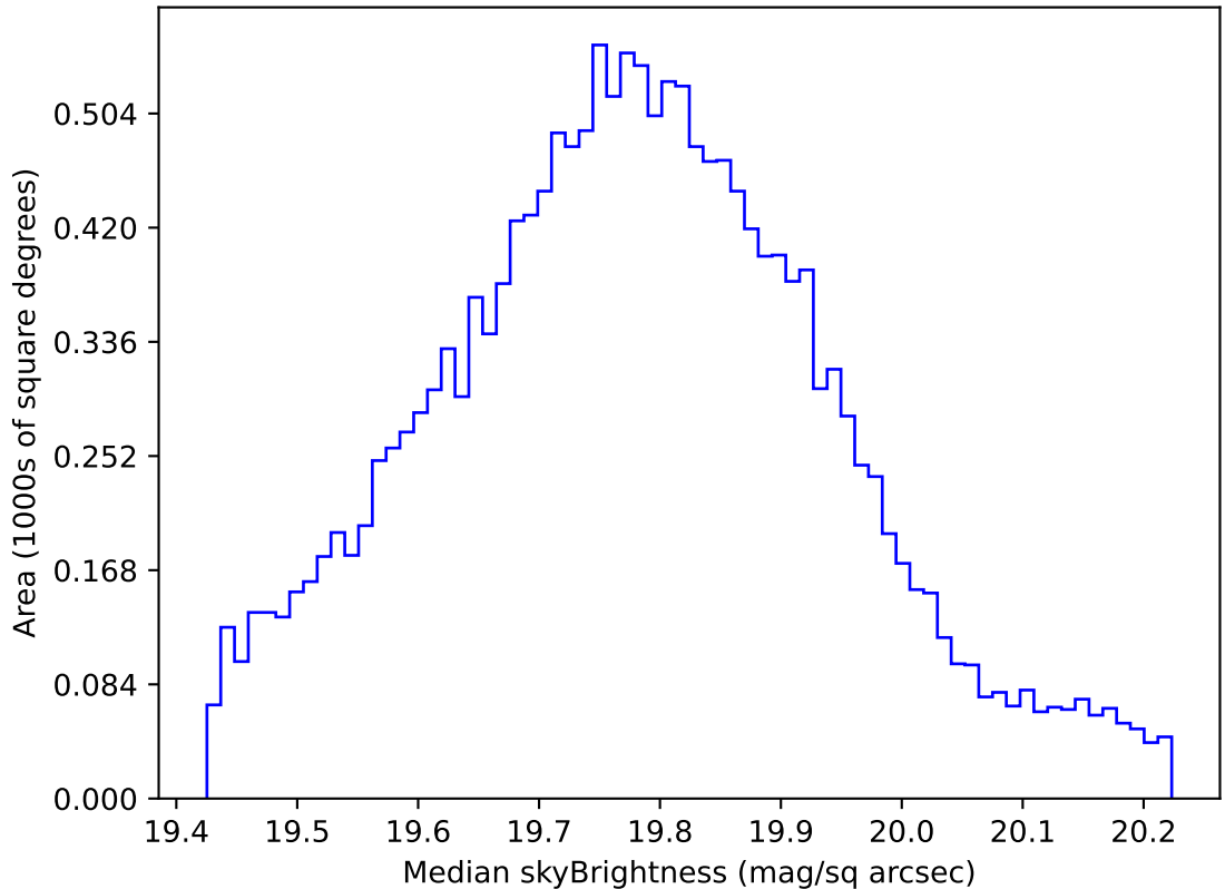
internal_u_expt30_nscale1.1v3.4_10yrs WFD all bands: Median skyBrightness
