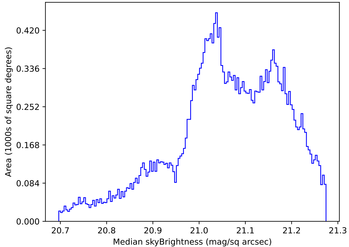
internal_u_expt30_nscale1.1v3.4_10yrs All sky r band: Median skyBrightness
