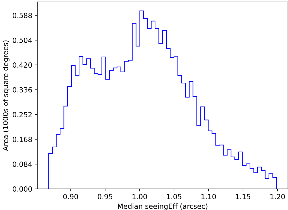
internal_u_expt30_nscale1.1v3.4_10yrs WFD z band: Median seeingEff
