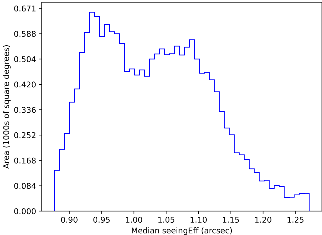
internal_u_expt30_nscale1.1v3.4_10yrs WFD r band: Median seeingEff
