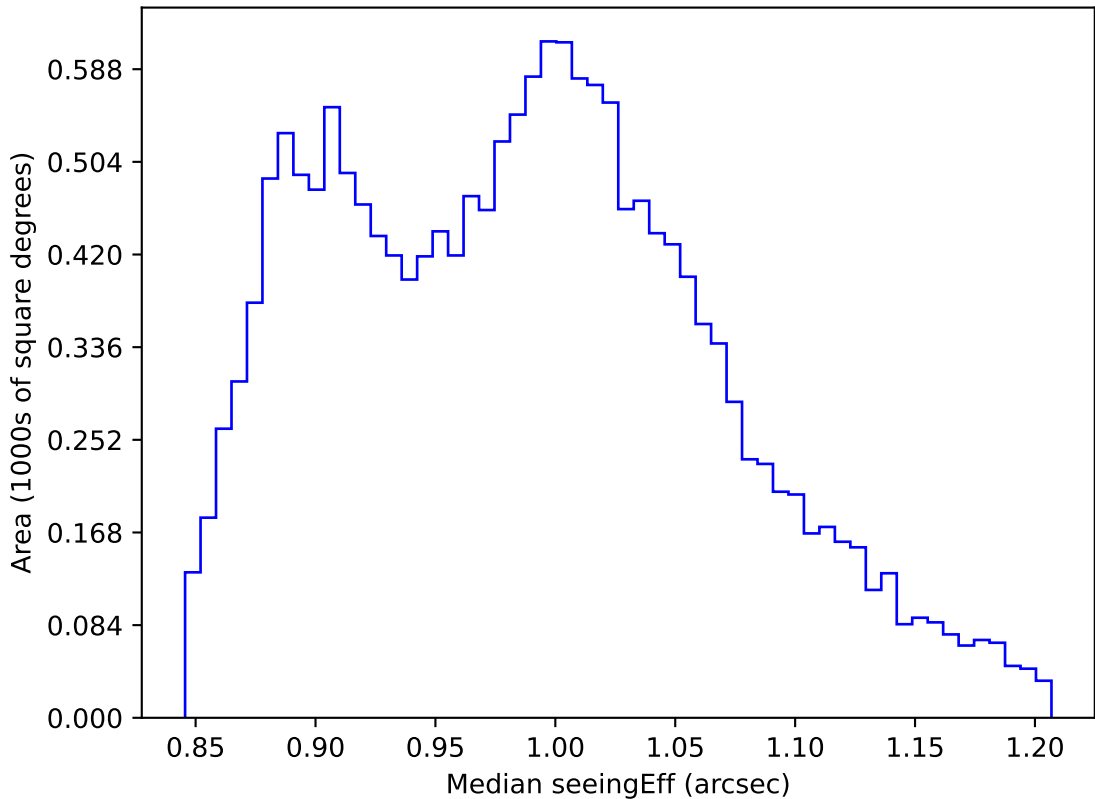
internal_u_expt30_nscale1.1v3.4_10yrs WFD i band: Median seeingEff
