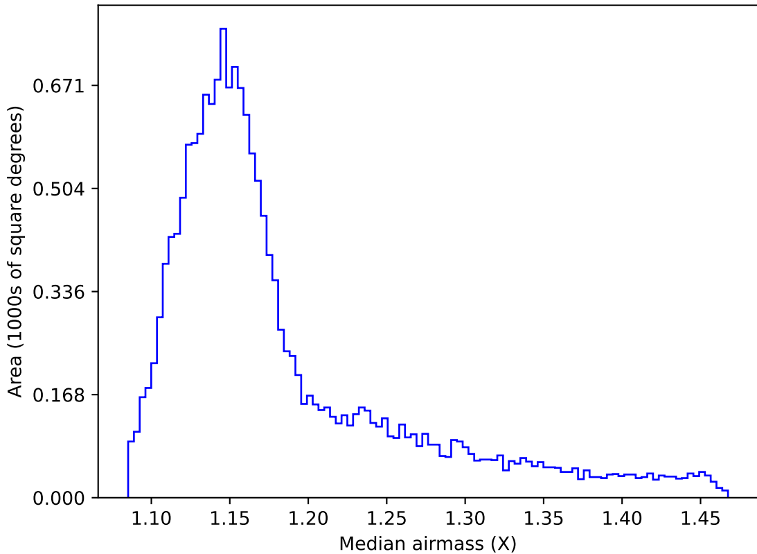
internal_u_expt30_nscale1.1v3.4_10yrs WFD z band: Median airmass
