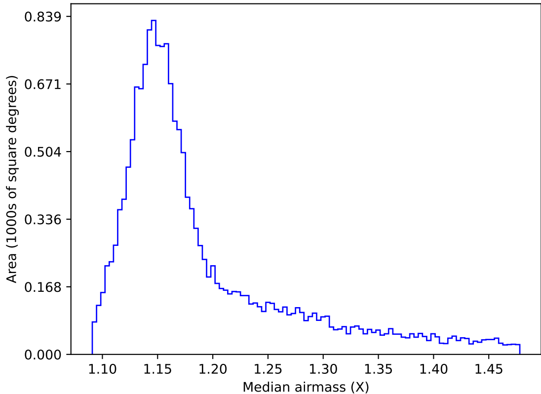
internal_u_expt30_nscale1.1v3.4_10yrs WFD y band: Median airmass
