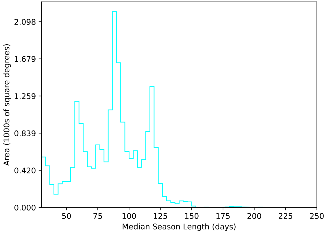
internal_u_expt30_nscale1.1v3.4_10yrs All sky u band: Median Season Length
