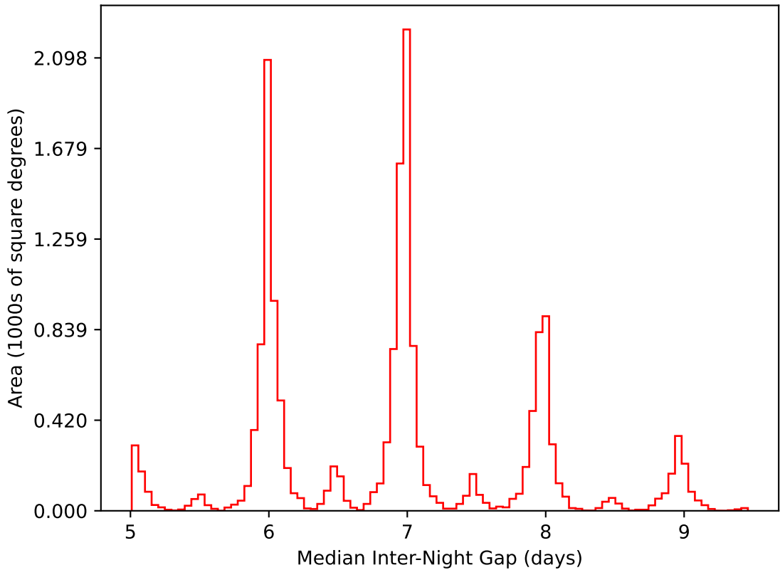
internal_u_expt30_nscale1.1v3.4_10yrs WFD i band: Median Inter-Night Gap
