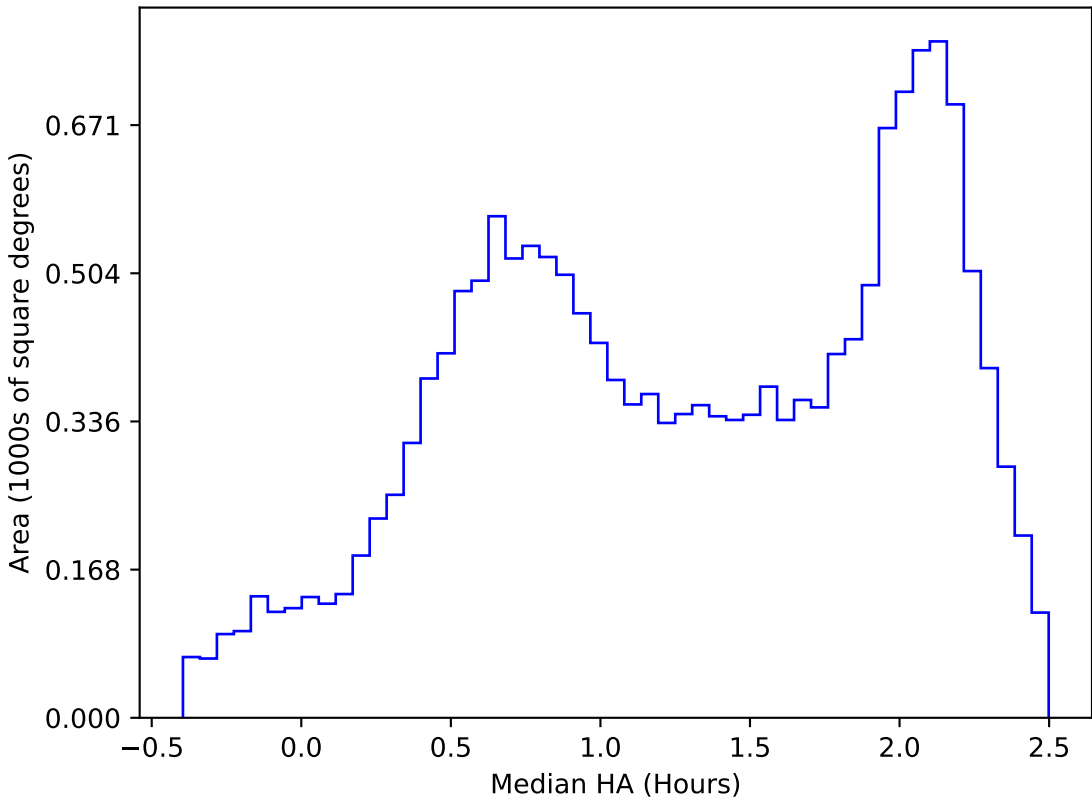
internal_u_expt30_nscale1.1v3.4_10yrs WFD y band: Median HA
