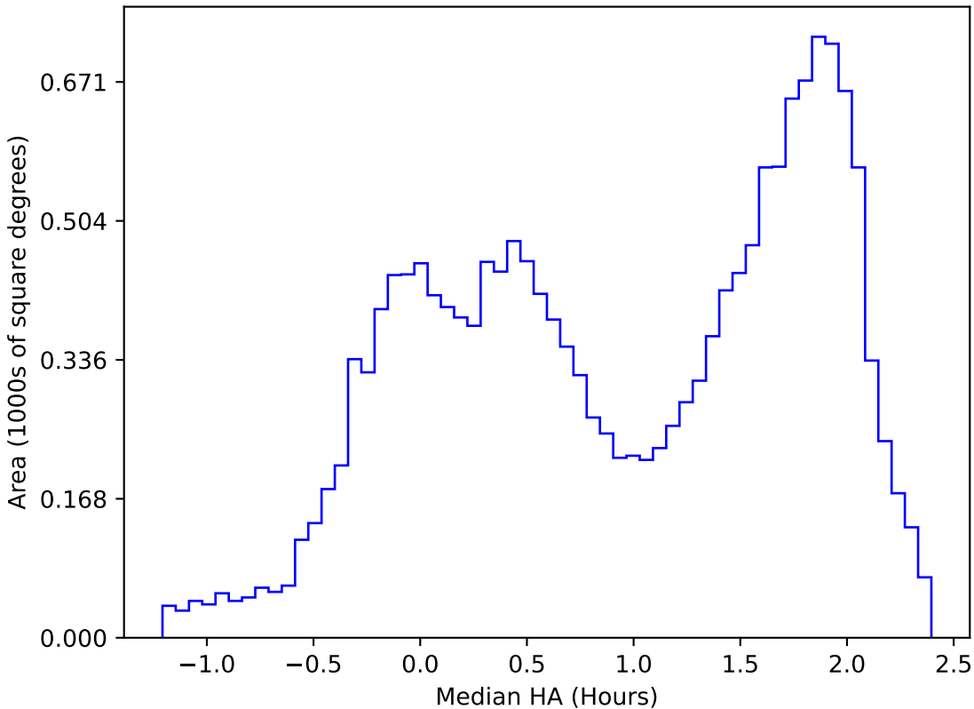
internal_u_expt30_nscale1.1v3.4_10yrs WFD u band: Median HA
