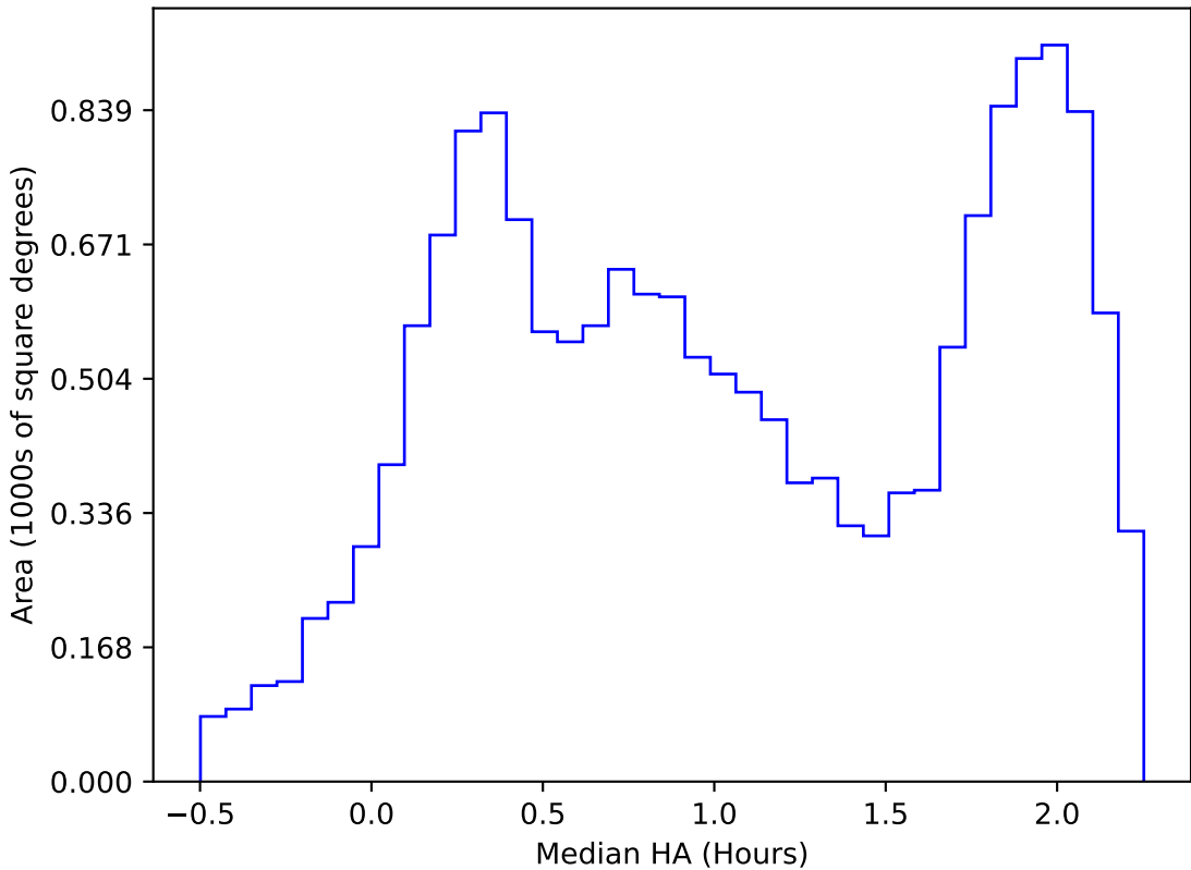
internal_u_expt30_nscale1.1v3.4_10yrs WFD i band: Median HA
