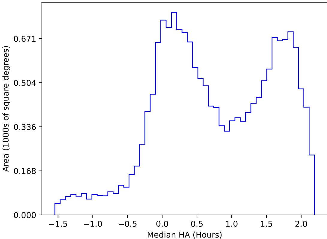
internal_u_expt30_nscale1.1v3.4_10yrs WFD g band: Median HA
