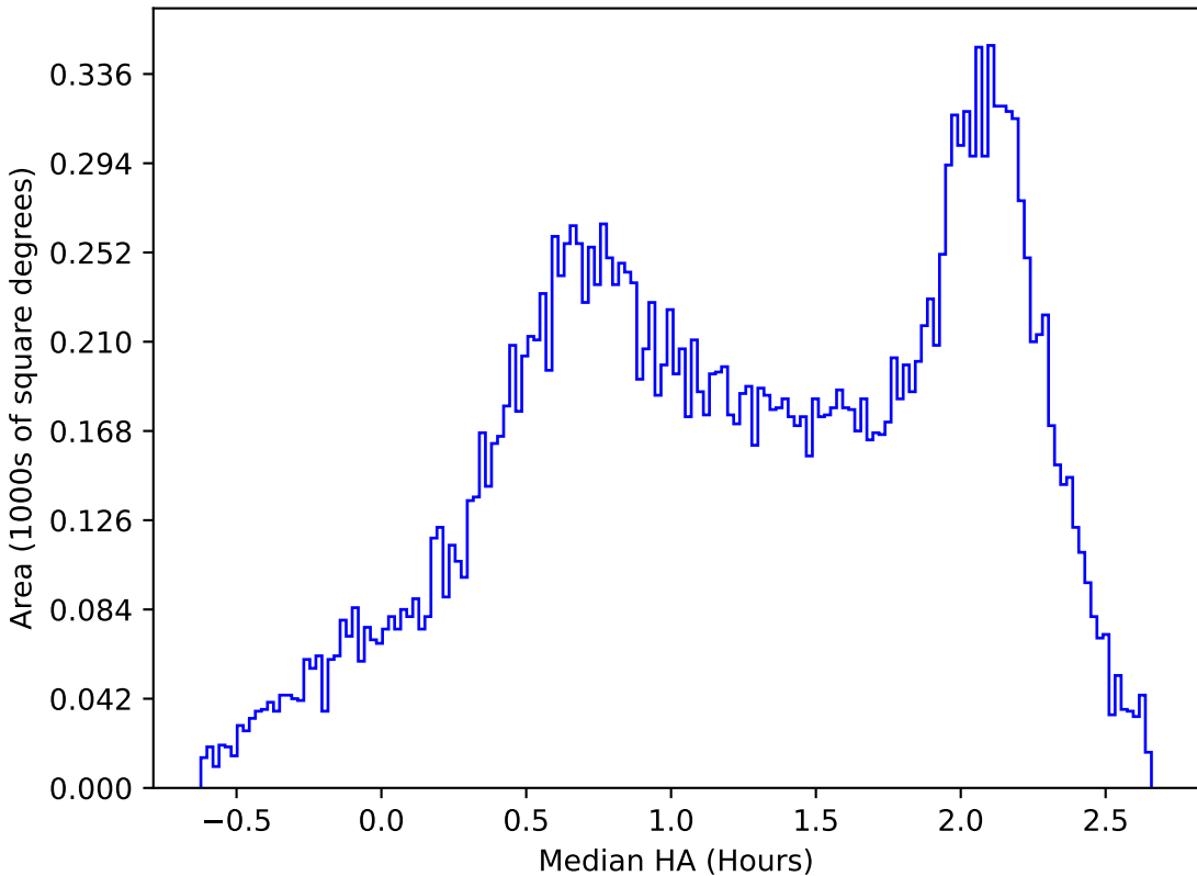
internal_u_expt30_nscale1.1v3.4_10yrs All sky y band: Median HA
