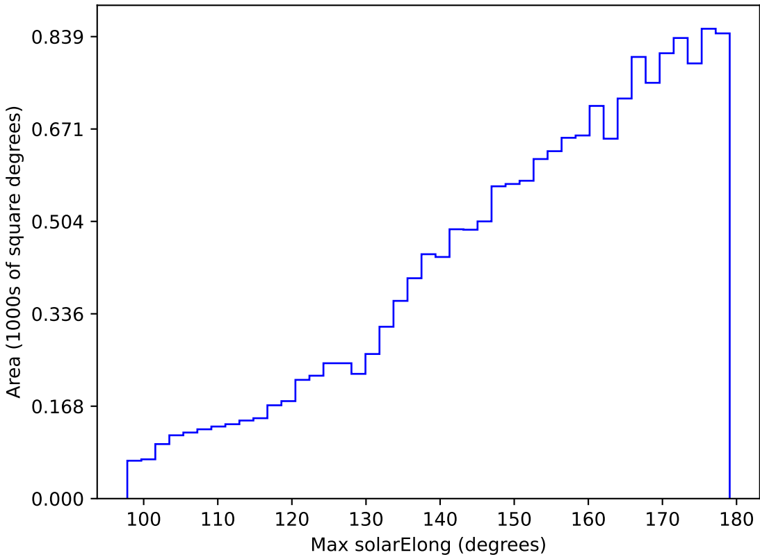
internal_u_expt30_nscale1.1v3.4_10yrs WFD u band: Max solarElong
