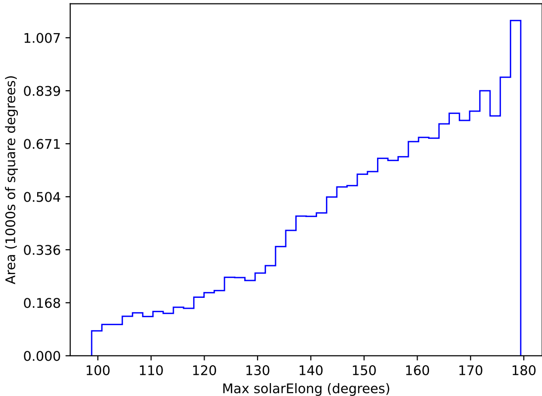
internal_u_expt30_nscale1.1v3.4_10yrs WFD r band: Max solarElong
