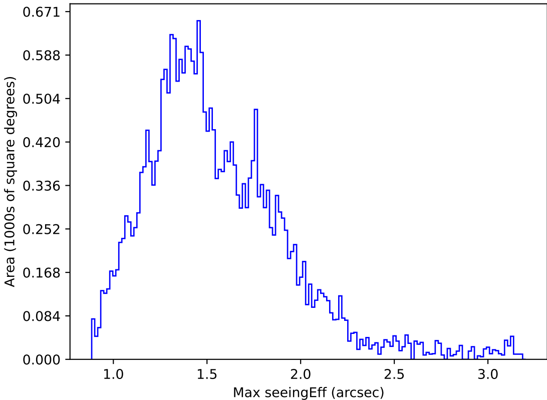
internal_u_expt30_nscale1.1v3.4_10yrs Yr 1 i band: Max seeingEff
