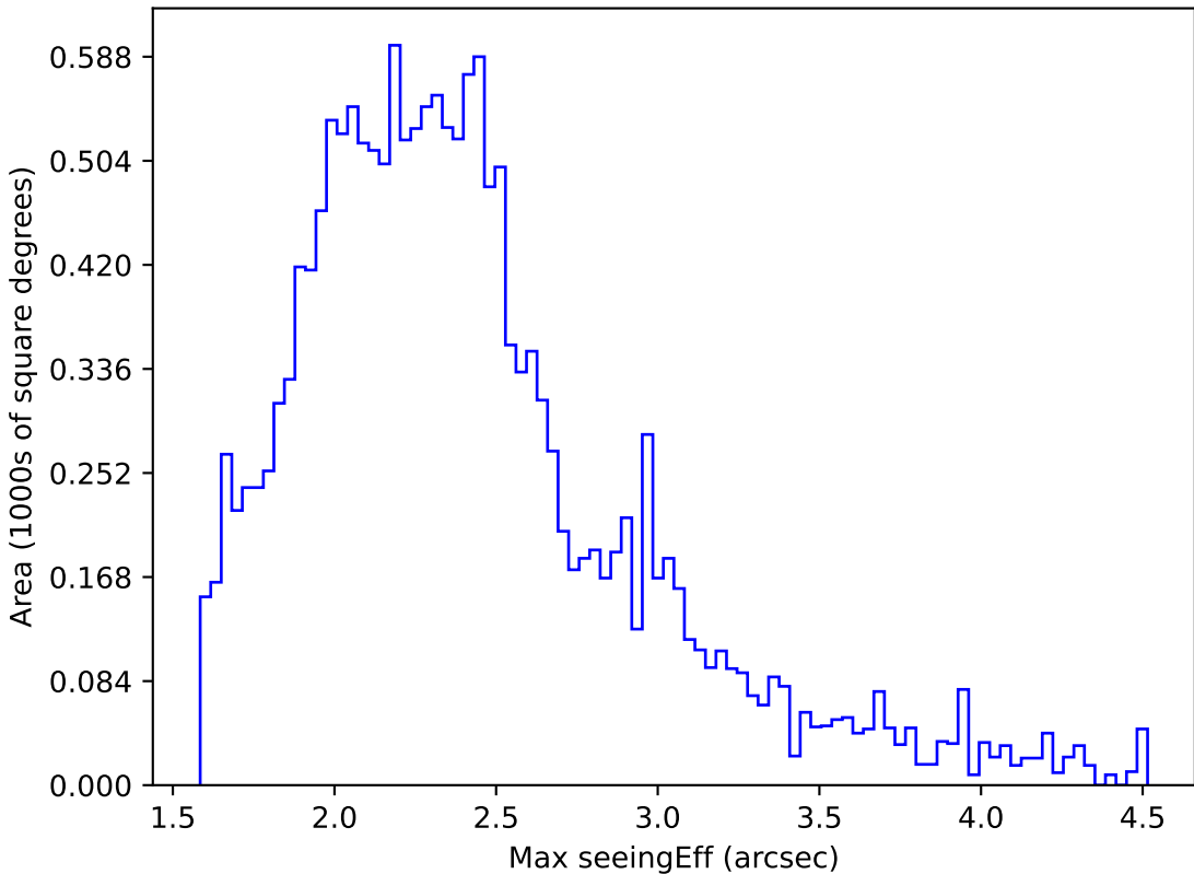
internal_u_expt30_nscale1.1v3.4_10yrs WFD y band: Max seeingEff
