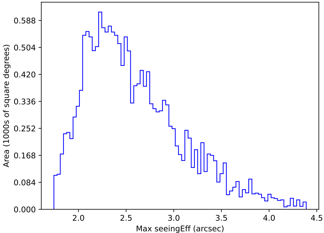
internal_u_expt30_nscale1.1v3.4_10yrs WFD u band: Max seeingEff
