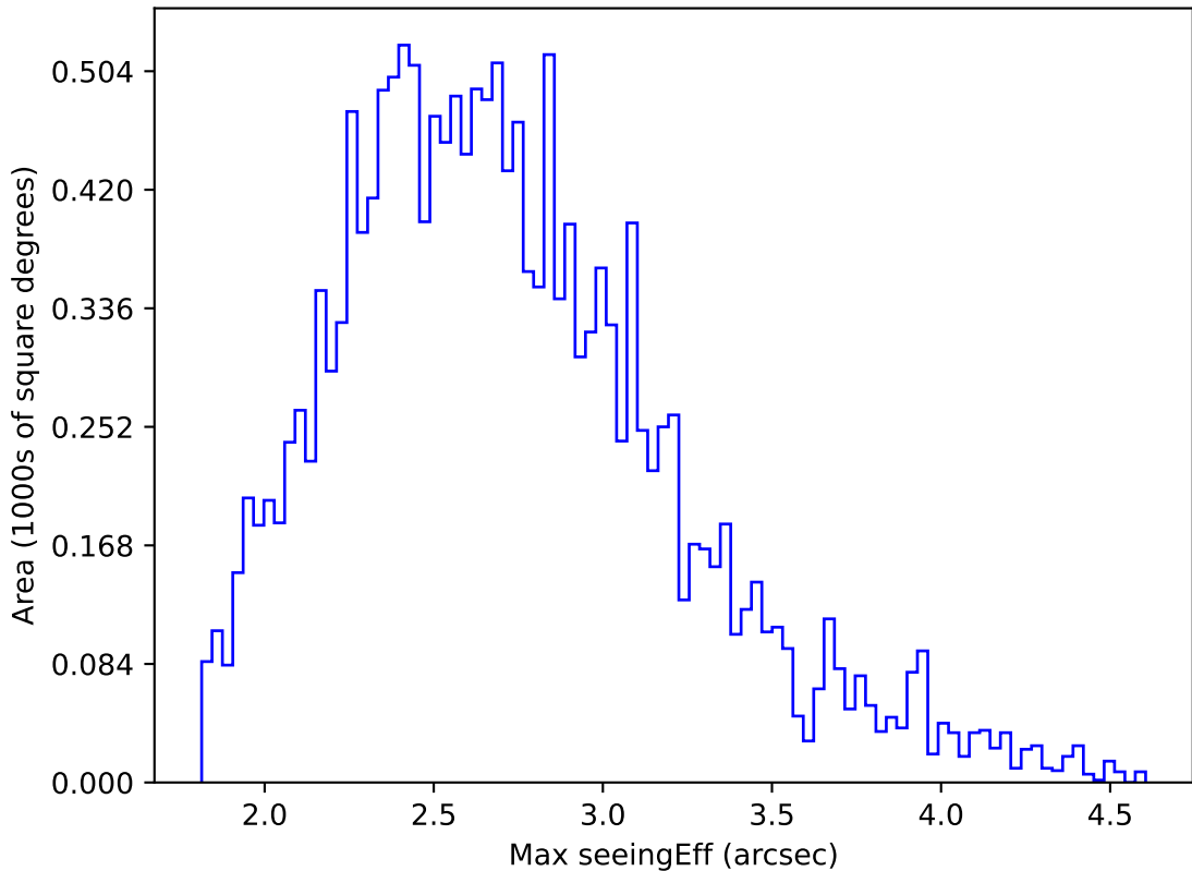
internal_u_expt30_nscale1.1v3.4_10yrs WFD r band: Max seeingEff
