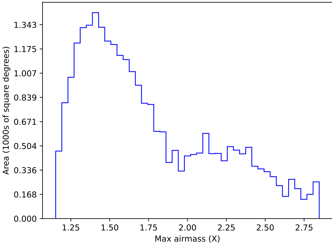
internal_u_expt30_nscale1.1v3.4_10yrs Yr 1 z band: Max airmass
