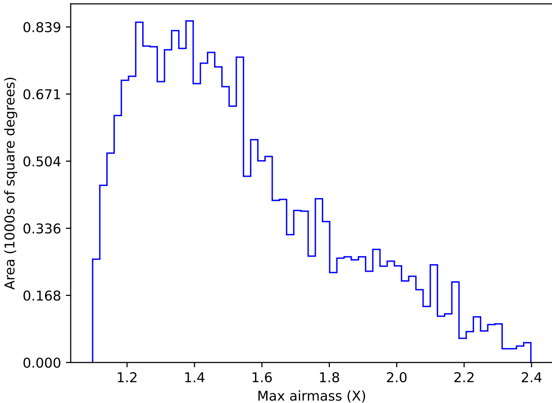
internal_u_expt30_nscale1.1v3.4_10yrs Yr 1 u band: Max airmass
