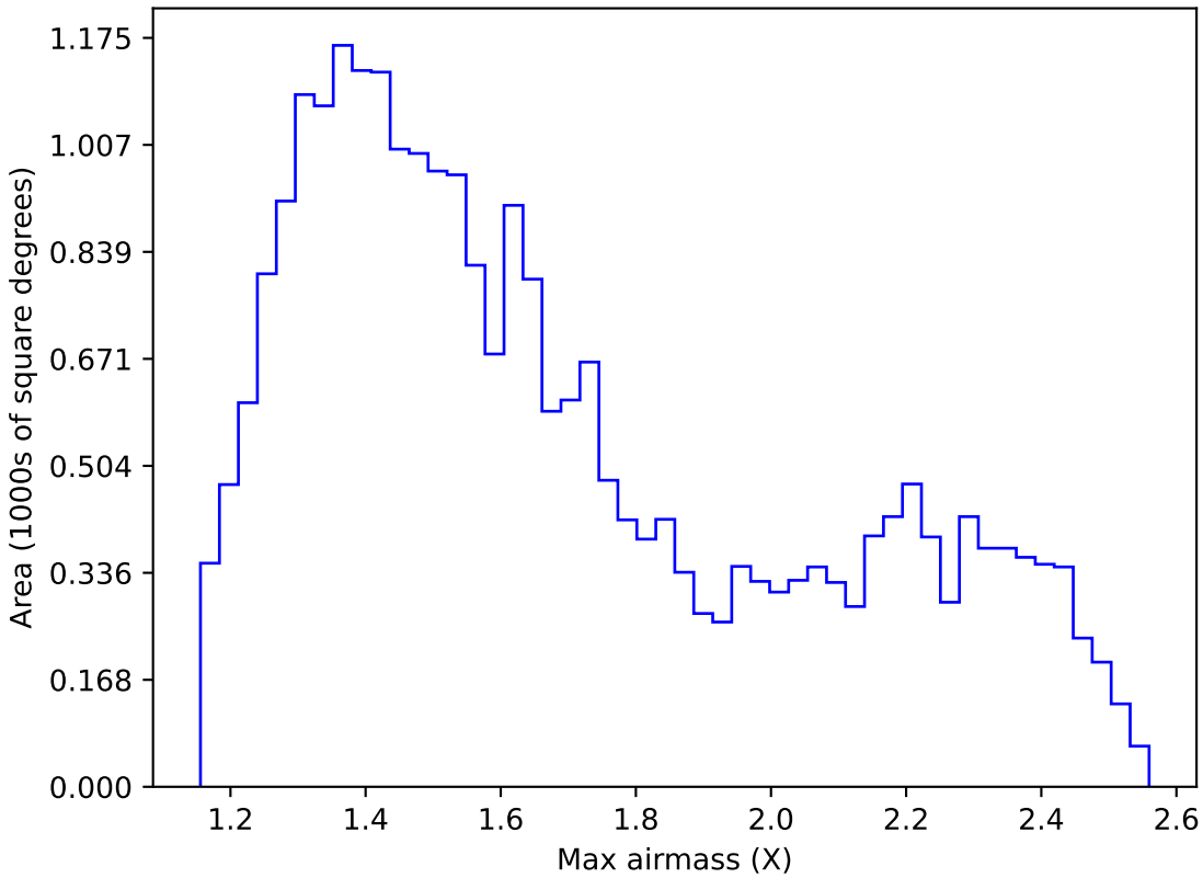
internal_u_expt30_nscale1.1v3.4_10yrs Yr 1 r band: Max airmass
