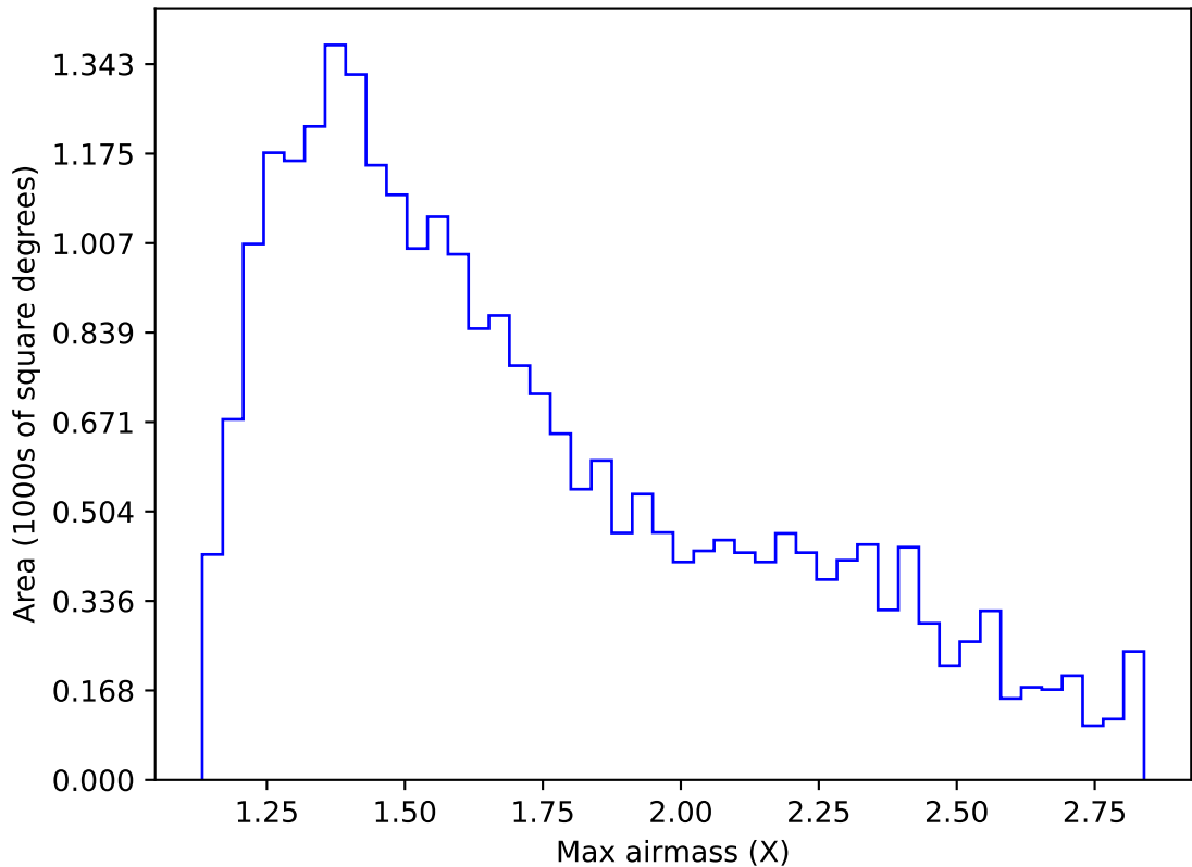
internal_u_expt30_nscale1.1v3.4_10yrs Yr 1 i band: Max airmass
