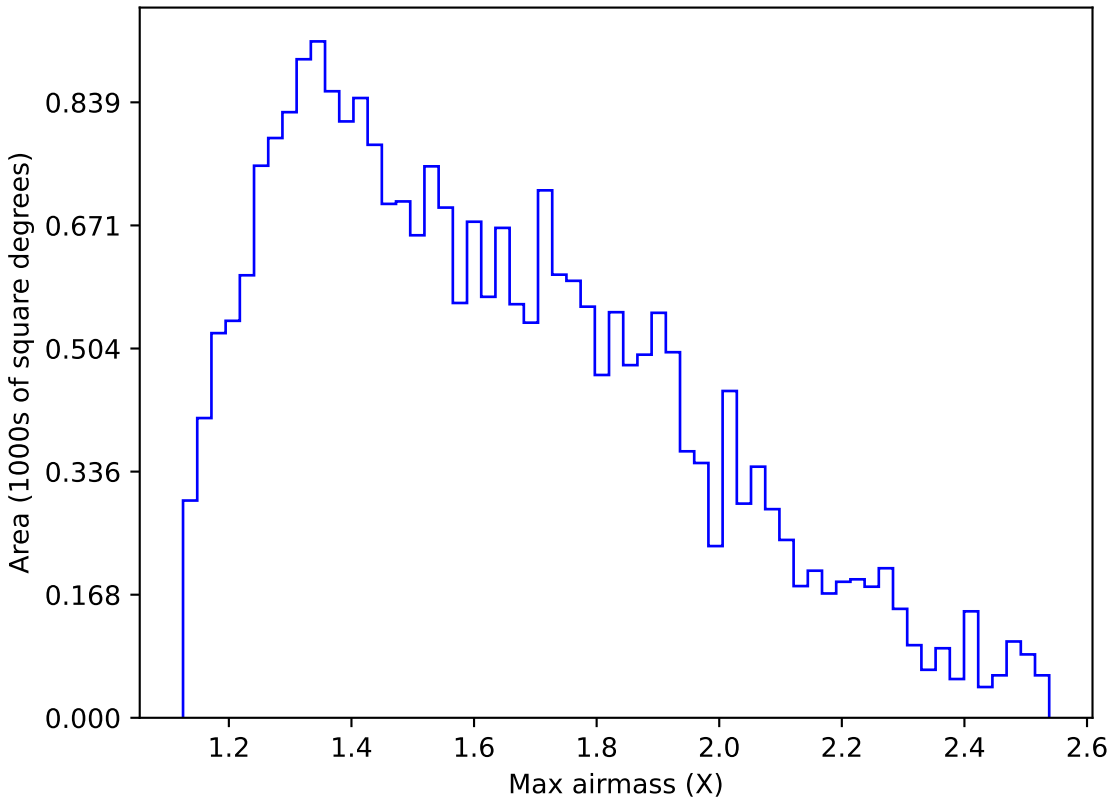
internal_u_expt30_nscale1.1v3.4_10yrs Yr 1 g band: Max airmass
