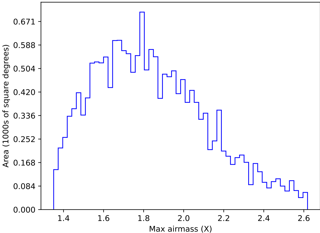
internal_u_expt30_nscale1.1v3.4_10yrs WFD u band: Max airmass
