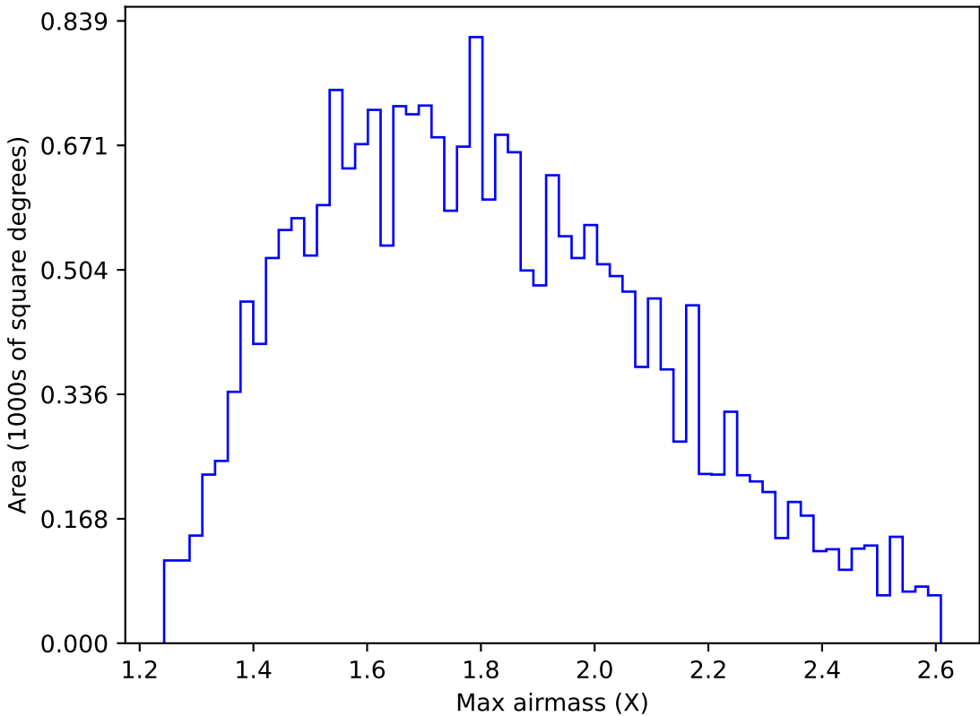
internal_u_expt30_nscale1.1v3.4_10yrs All sky u band: Max airmass
