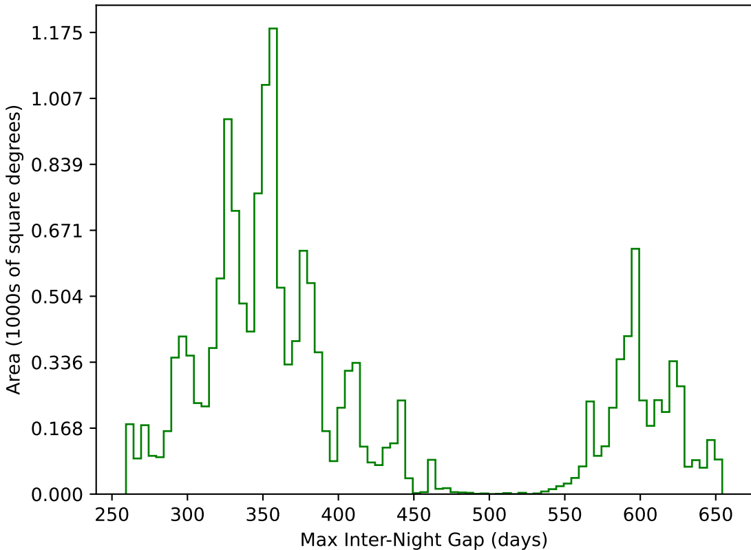
internal_u_expt30_nscale1.1v3.4_10yrs WFD g band: Max Inter-Night Gap
