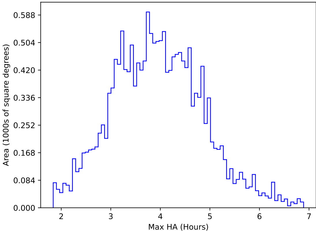
internal_u_expt30_nscale1.1v3.4_10yrs WFD u band: Max HA
