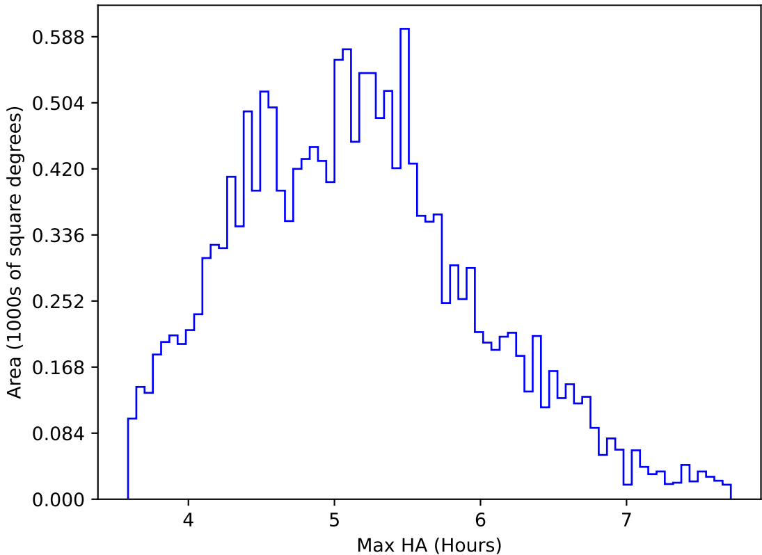
internal_u_expt30_nscale1.1v3.4_10yrs WFD all bands: Max HA
