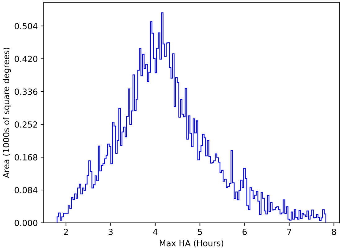
internal_u_expt30_nscale1.1v3.4_10yrs All sky r band: Max HA
