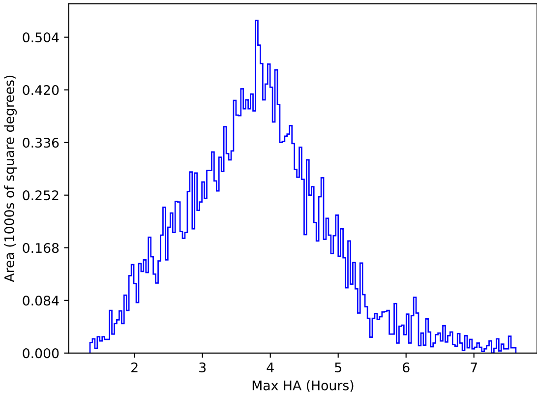
internal_u_expt30_nscale1.1v3.4_10yrs All sky g band: Max HA
