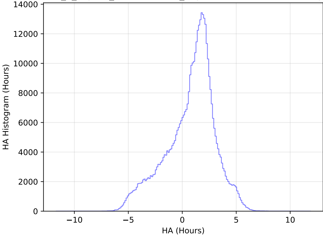
internal_u_expt30_nscale1.1v3.4_10yrs WFD z band: HA Histogram
