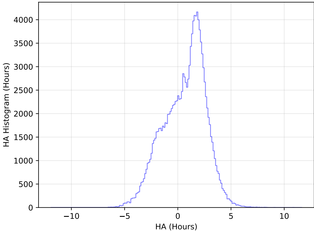
internal_u_expt30_nscale1.1v3.4_10yrs WFD u band: HA Histogram
