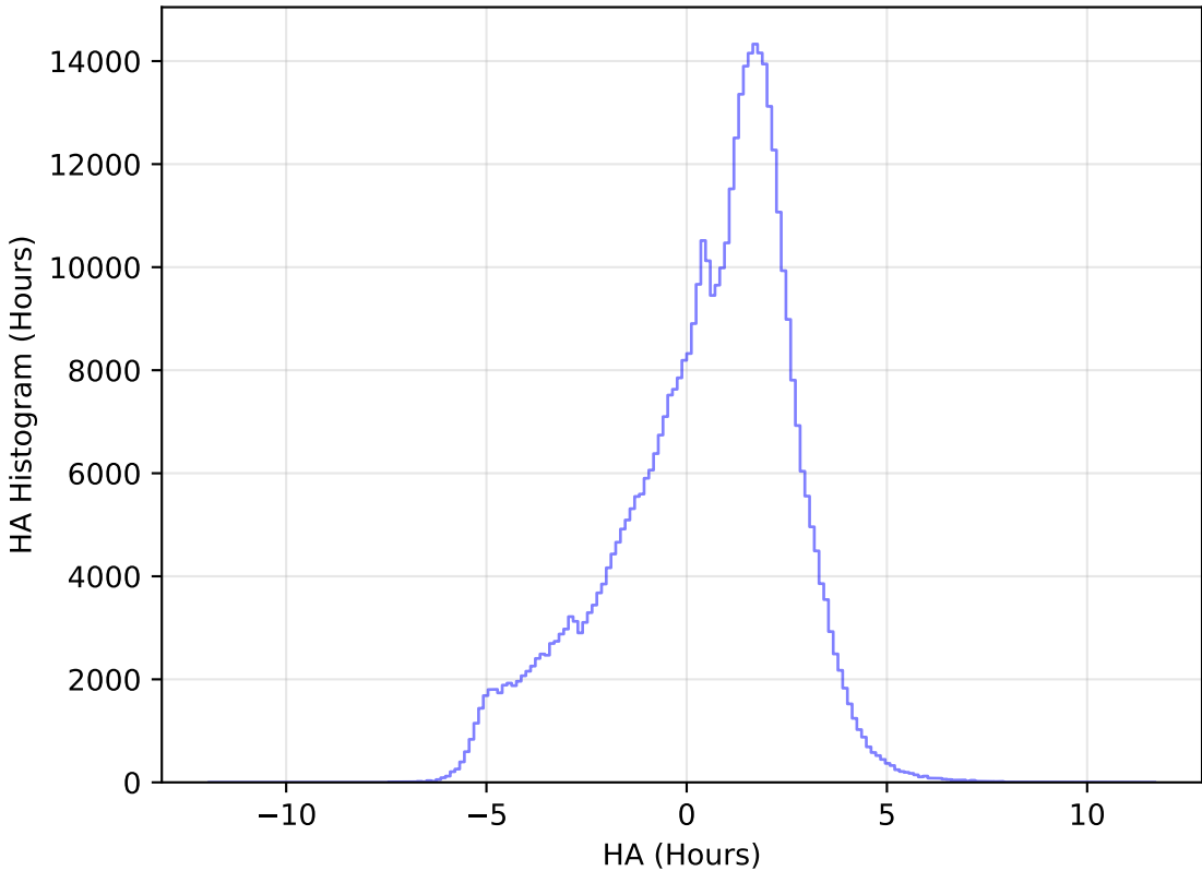
internal_u_expt30_nscale1.1v3.4_10yrs WFD r band: HA Histogram
