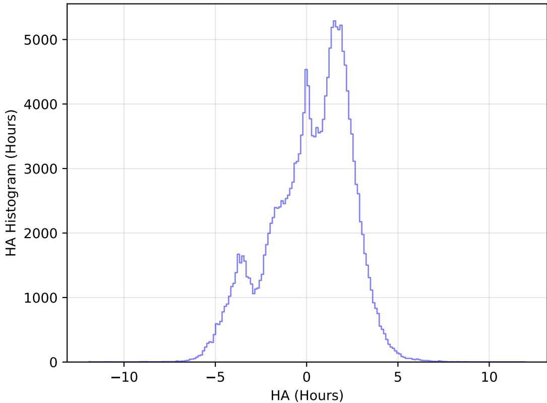
internal_u_expt30_nscale1.1v3.4_10yrs WFD g band: HA Histogram
