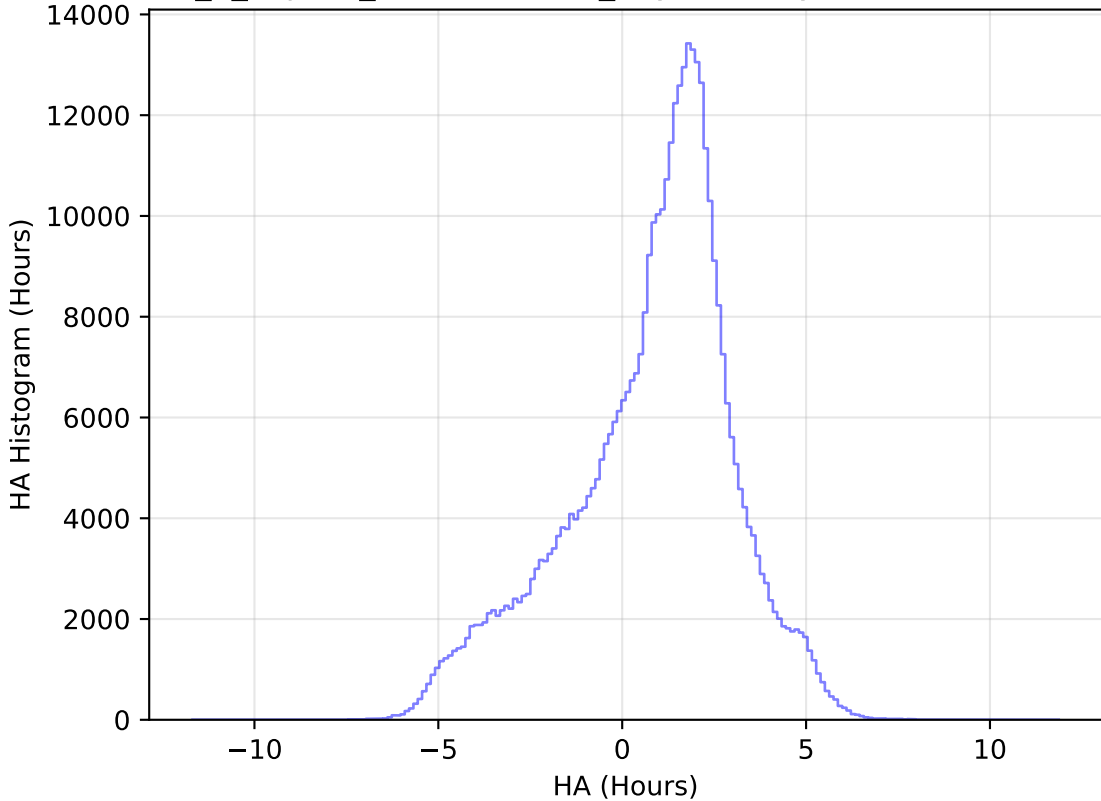
internal_u_expt30_nscale1.1v3.4_10yrs All sky z band: HA Histogram
