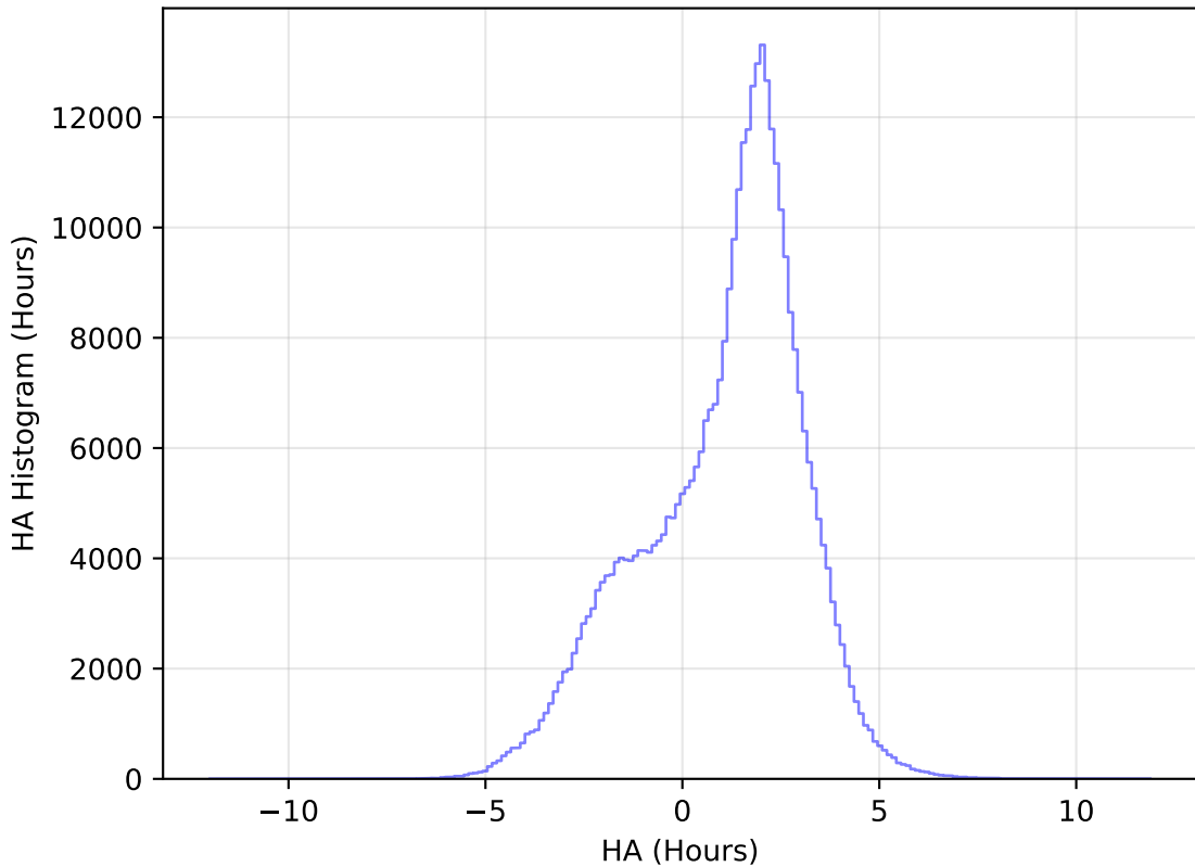
internal_u_expt30_nscale1.1v3.4_10yrs All sky y band: HA Histogram
