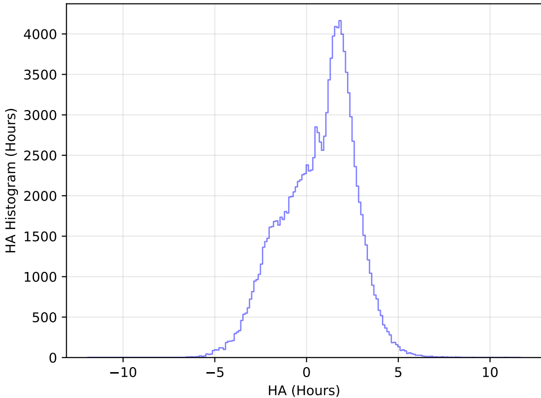
internal_u_expt30_nscale1.1v3.4_10yrs All sky u band: HA Histogram
