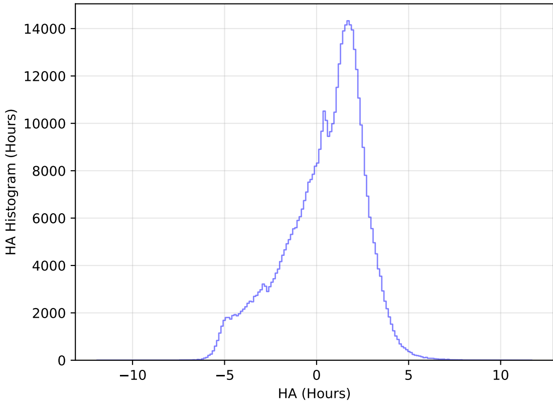
internal_u_expt30_nscale1.1v3.4_10yrs All sky r band: HA Histogram
