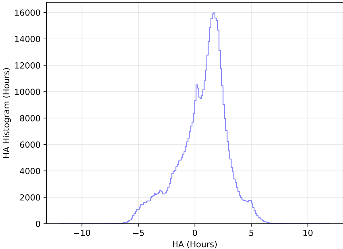
internal_u_expt30_nscale1.1v3.4_10yrs All sky i band: HA Histogram
