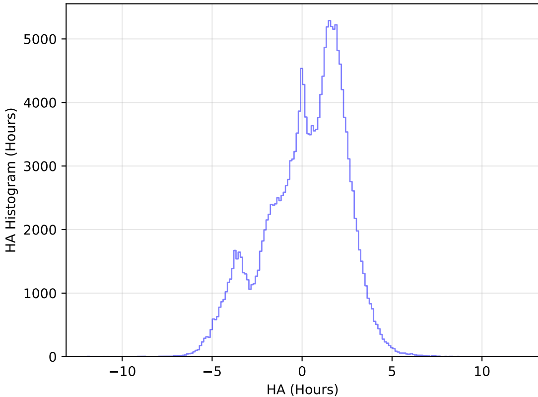
internal_u_expt30_nscale1.1v3.4_10yrs All sky g band: HA Histogram
