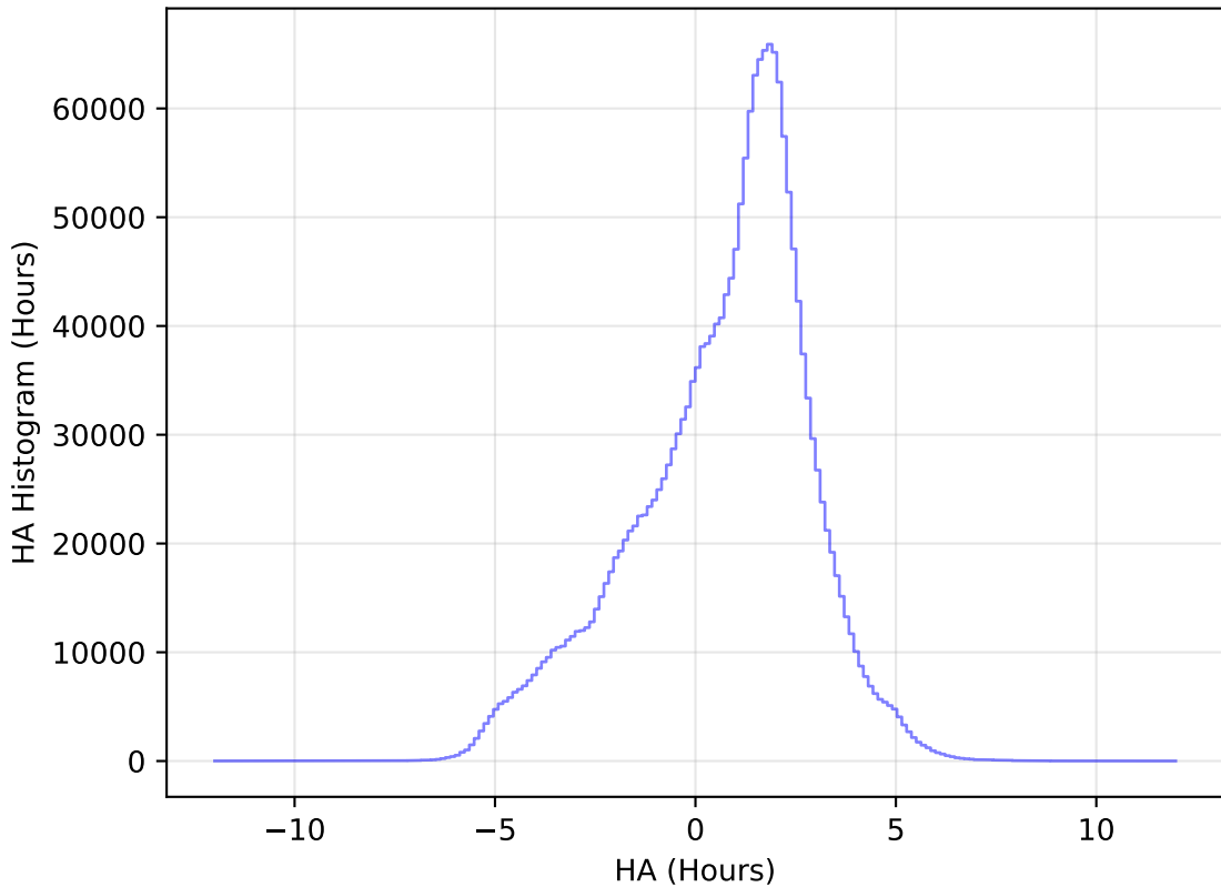
internal_u_expt30_nscale1.1v3.4_10yrs All sky all bands: HA Histogram
