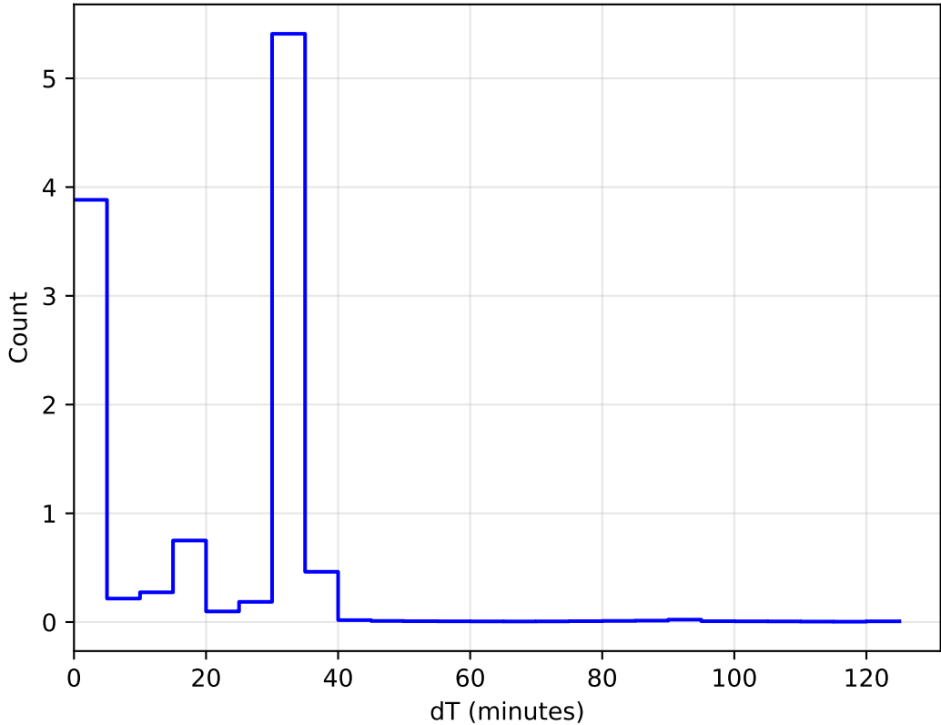
internal_u_expt30_nscale1.1v3.4_10yrs WFD: DeltaT Histogram
