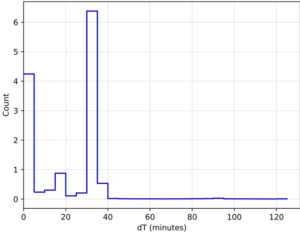
internal_u_expt30_nscale1.1v3.4_10yrs All sky: DeltaT Histogram 1e6
